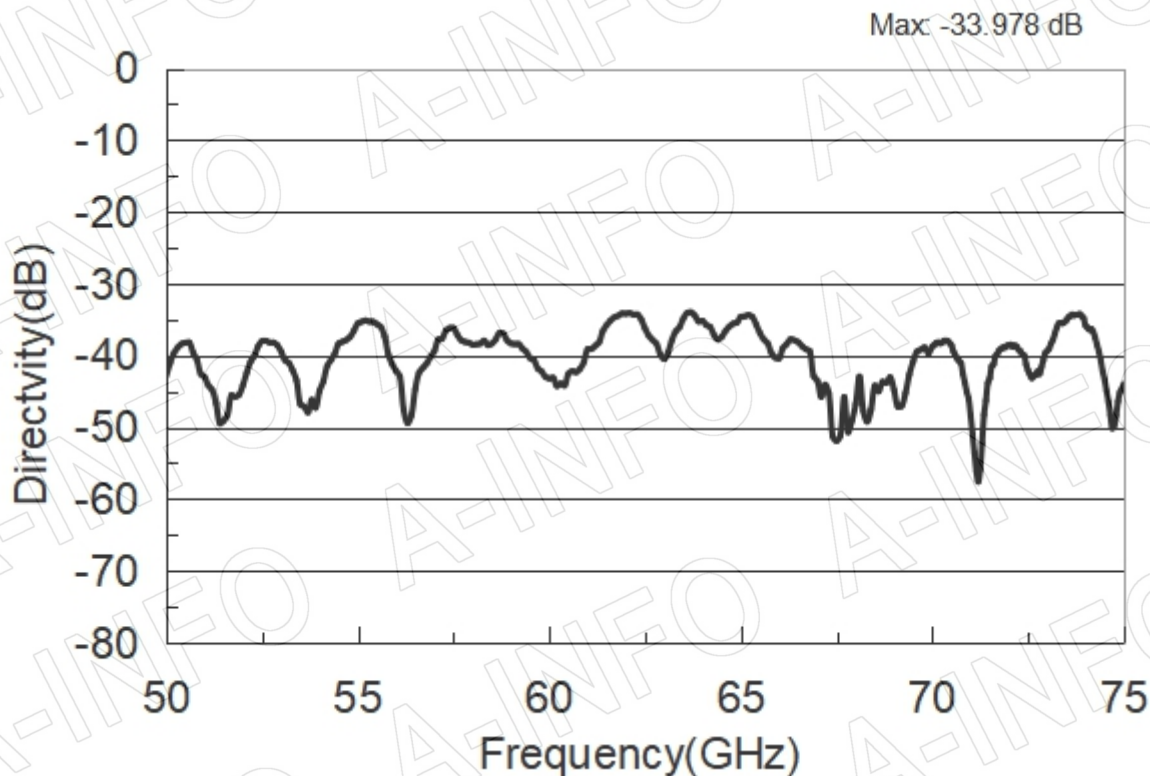
Directivity Port 1
